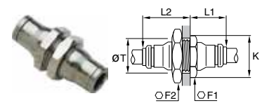
62PLMBH Bulkhead Connector Inch Tube to Tube
