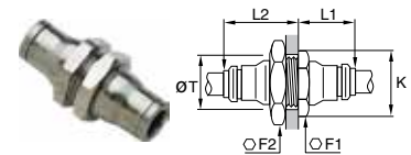
62PLMBH Bulkhead Connector Metric Tube to Tube
