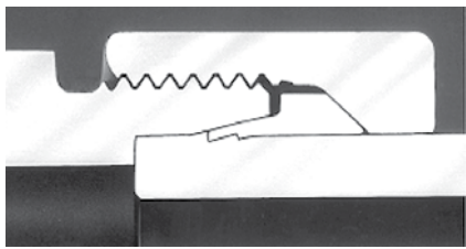
Profile ring – no deformation due to excessive tightening
