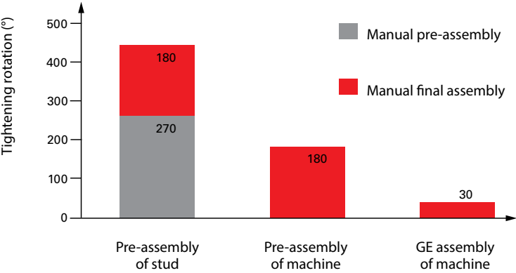
Tightening rotation comparison for Walpro-X
