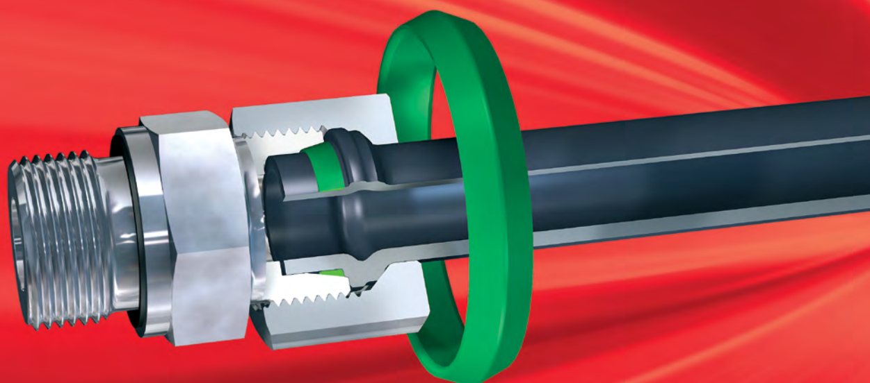
Assembly instructions for WalfarmPlus For steel or stainless steel (1.4571) tubes
