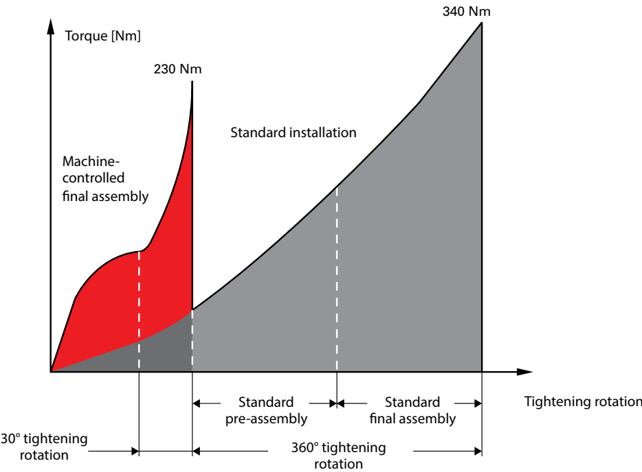
Comparison of assembly types
