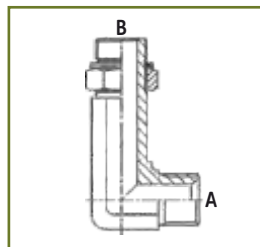
Long 90° adjustable stud adapter with o-ring and washer, thread BSP parallel
