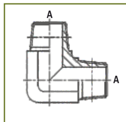
Male 90° adaptor, thread BSPT parallel
