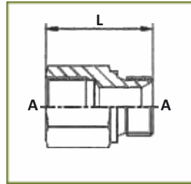
Male female straight adapter thread BSP parallel
