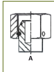
Female plug swivel BSP
