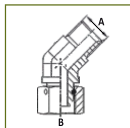
45° elbow adapter with swivel nut, thread BSP parallel
