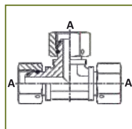
Branch tee adapter with swivel nuts, thread BSP parallel
