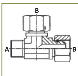
Male tee adapter with swivel nut, thread BSP parallel
