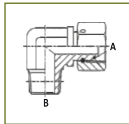
90° adapter with swivel nut BSP/ NPTF
