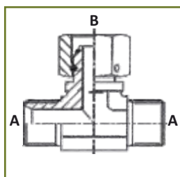
Branch tee adapter with swivel nut, thread BSP parallel
