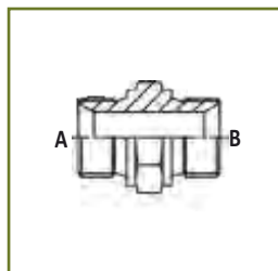
Male straight adapter thread metric parallel, cone 60° (reduction 1770-__)
