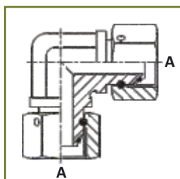
90° elbow adapter with double swivel nuts, thread BSP parallel
