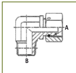
90° adapter with swivel nut BSP/ BSPT
