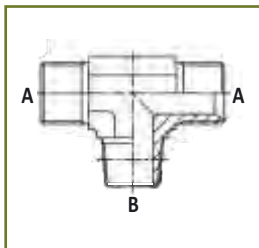
Male stud branch tee adapter BSP/ BSPT
