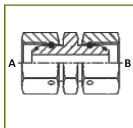
Straight adapter with double swivel nuts, thread BSP parallel
