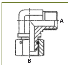
90° adapter with swivel nut, thread BSP parallel
