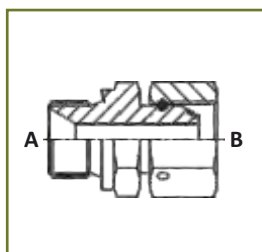
Straight adapter with swivel nut, thread BSP parallel
