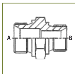
Male straight adapter BSP parallel and metric (cone 60°)
