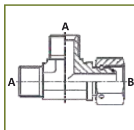
Barrel tee adapter with swivel nut, thread BSP parallel
