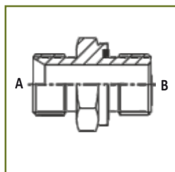
Male stud adapter with elastomer seal, thread BSP parallel
