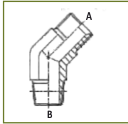
Male stud 45° adapter BSP/ NPTF
