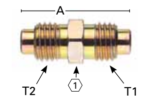
Union Adapter
