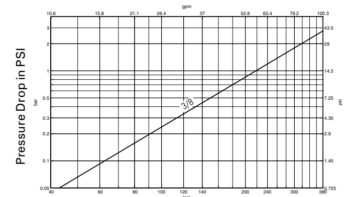
Gallons Per Minute Flow Test Fluid: Water at 70°F
