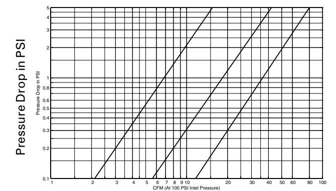
Cubic Feet Per Minute Flow Test Fluid: Air at 100 PSI Inlet Pressure
