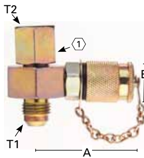
Swivel Run Tee with Test Coupling
